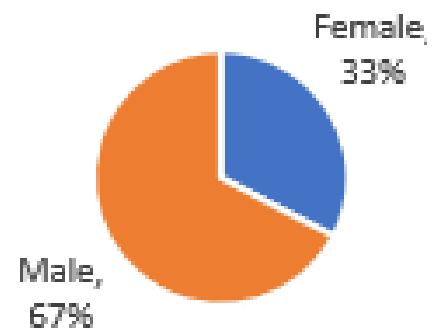
Lower Quartile
