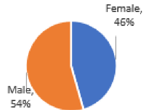
Upper Quartile
